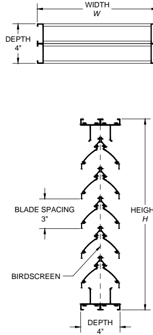
MODEL: 2440 FRAME: CHANNEL FRAME DUCT-MOUNT (DM)
