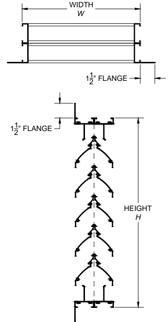
MODEL: 2445 FRAME: FLANGE FRAME FLANGE-MOUNT (FM)
